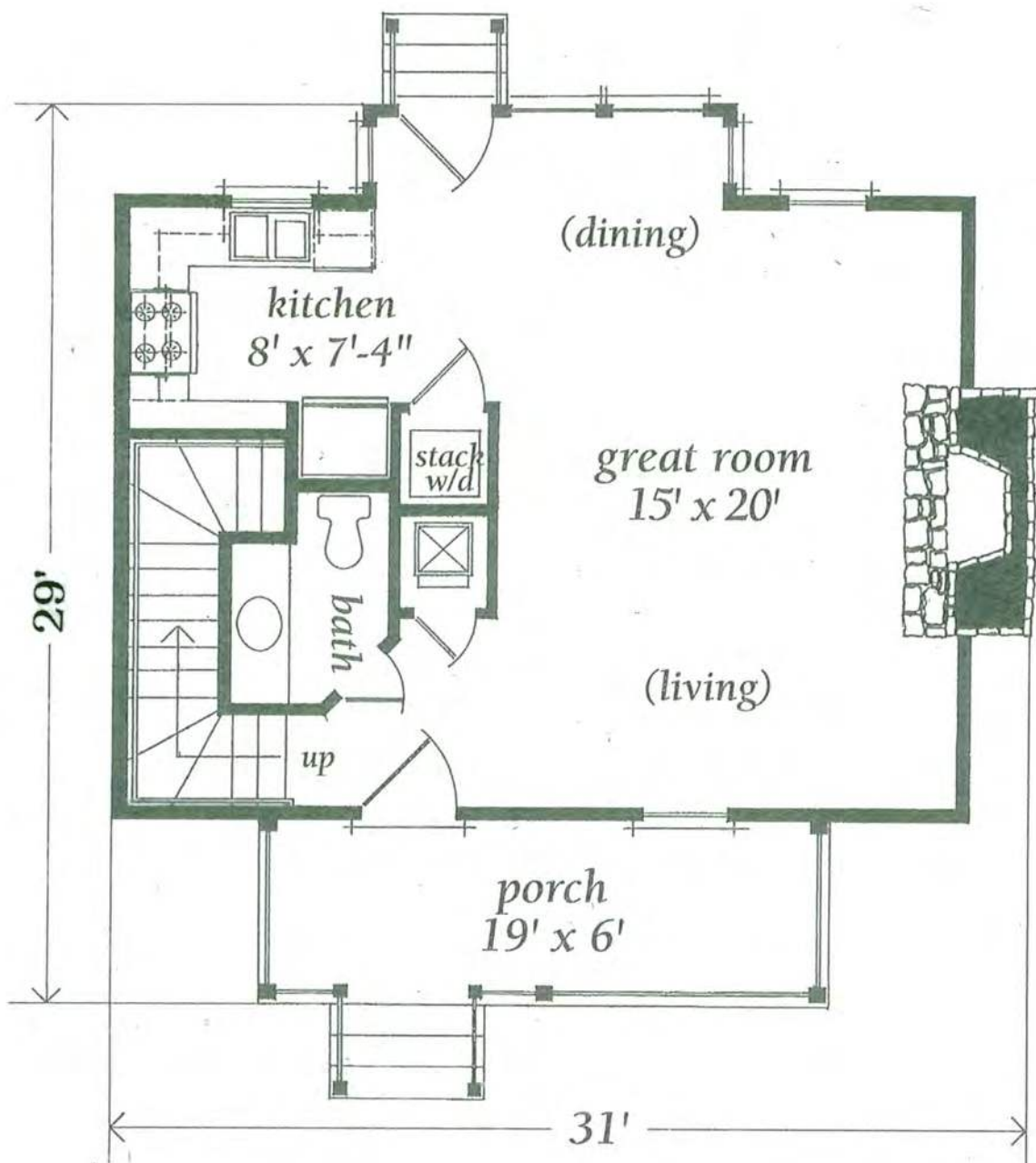
FIRST FLOOR (596 SQ. FT.)
