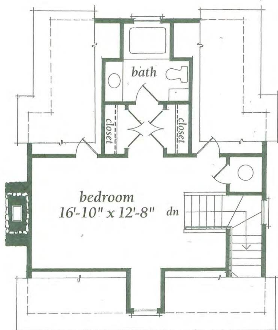
SECOND FLOOR (470 SQ. FT.)
