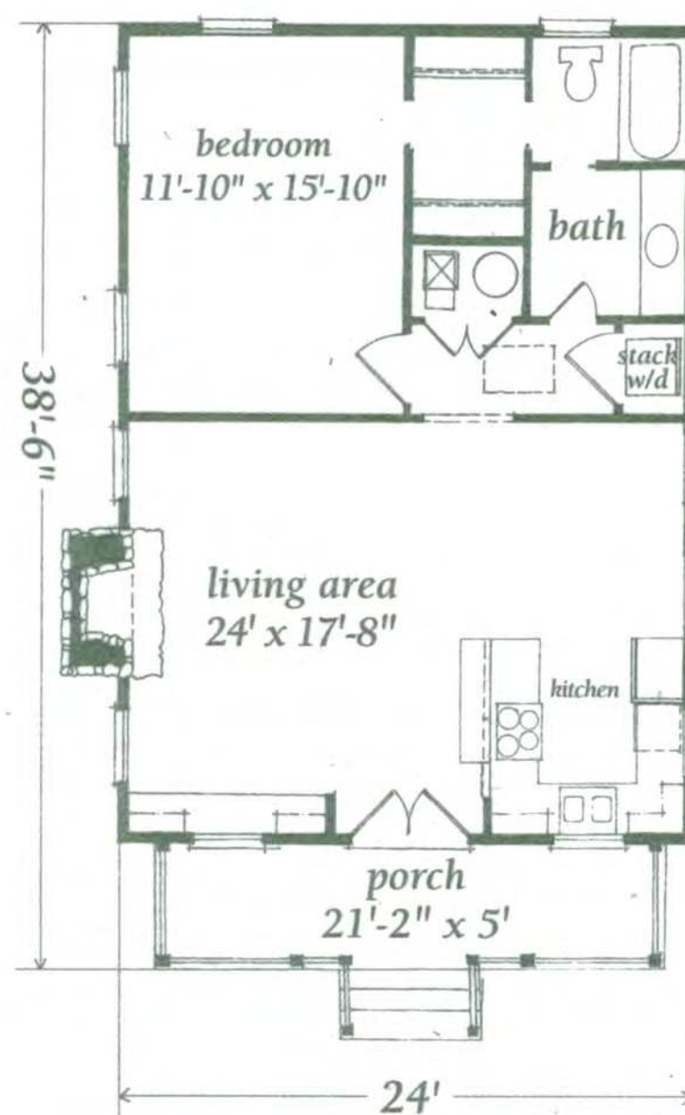
ALTERNATE FLOOR PLAN
