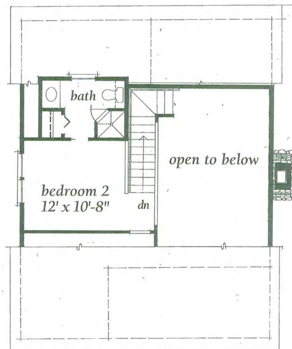
SECOND FLOOR (210 SQ. FT.)
