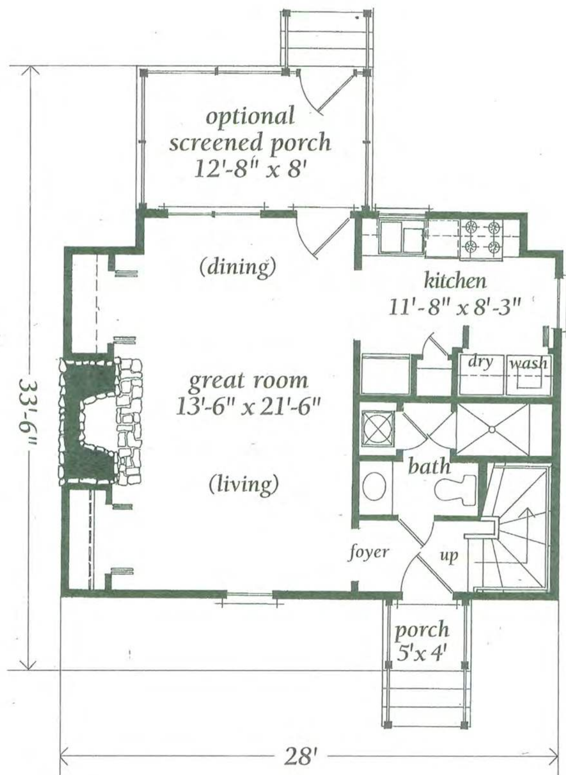
FIRST FLOOR (590 SQ. FT.)
