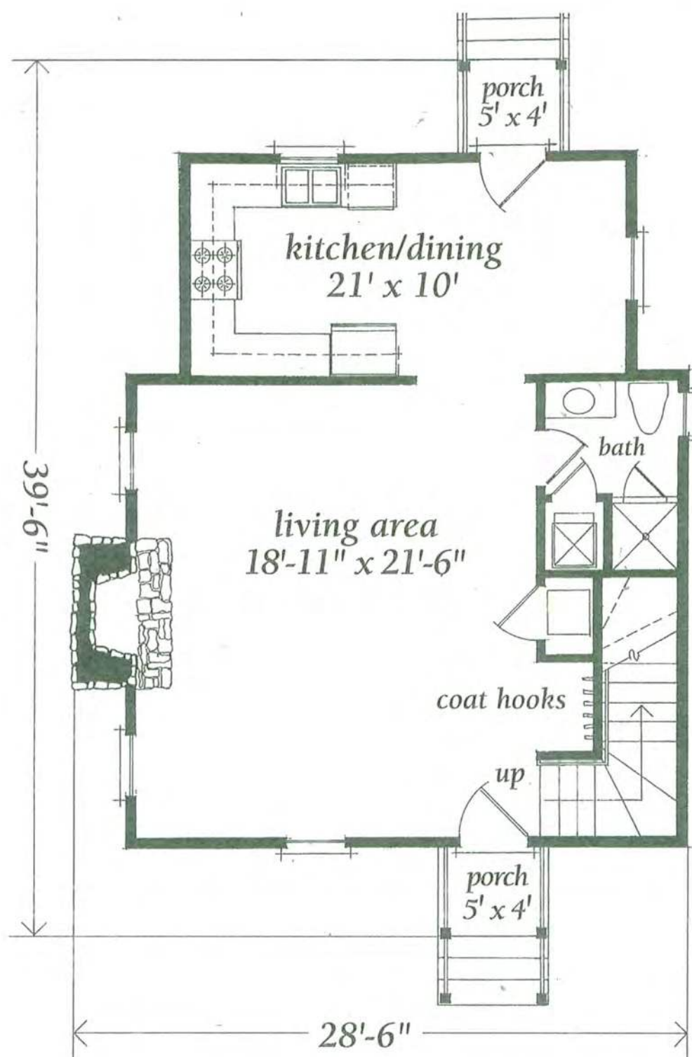
FIRST FLOOR (787 SQ. FT.)
