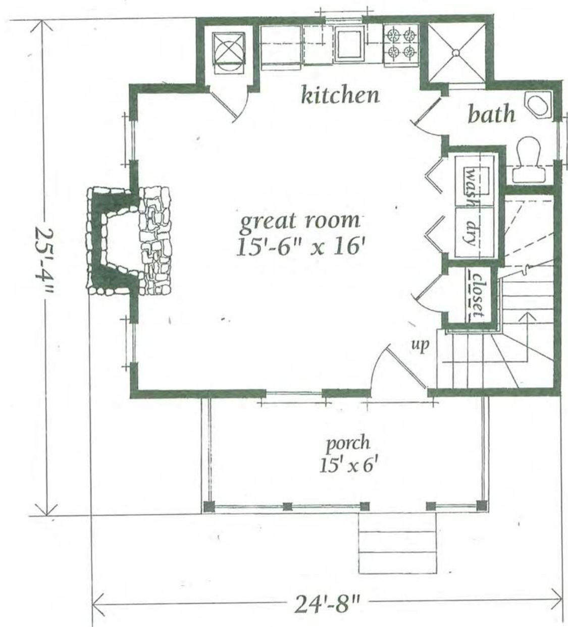
FIRST FLOOR (409 SQ. FT.)
