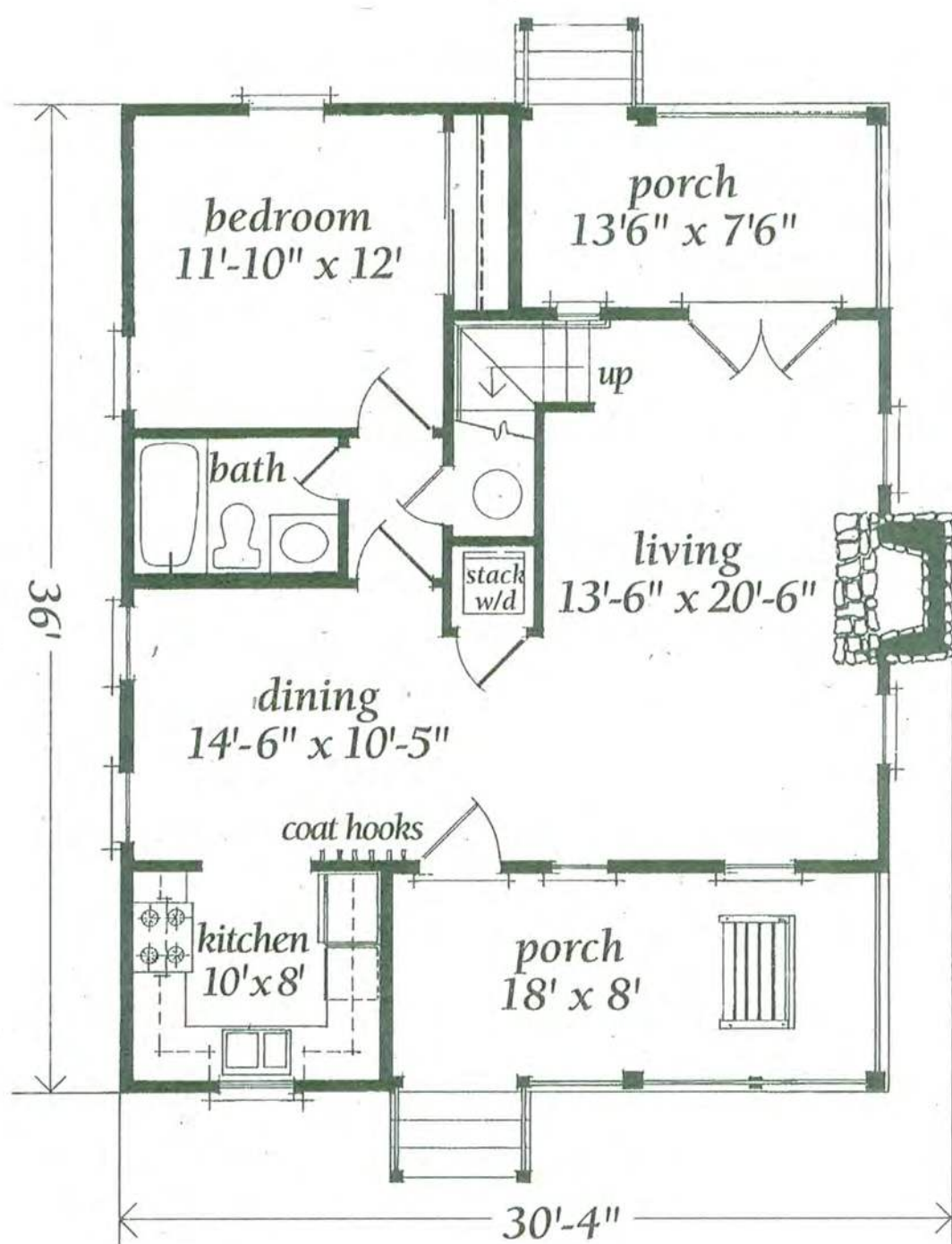
FIRST FLOOR (763 SQ. FT.)
