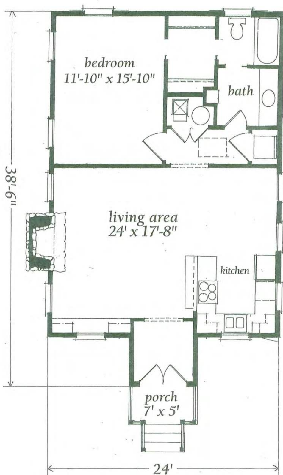
FLOOR PLAN AS SHOWN IN RENDERING
