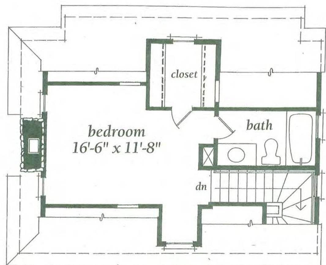
SECOND FLOOR (307 SQ. FT.)
