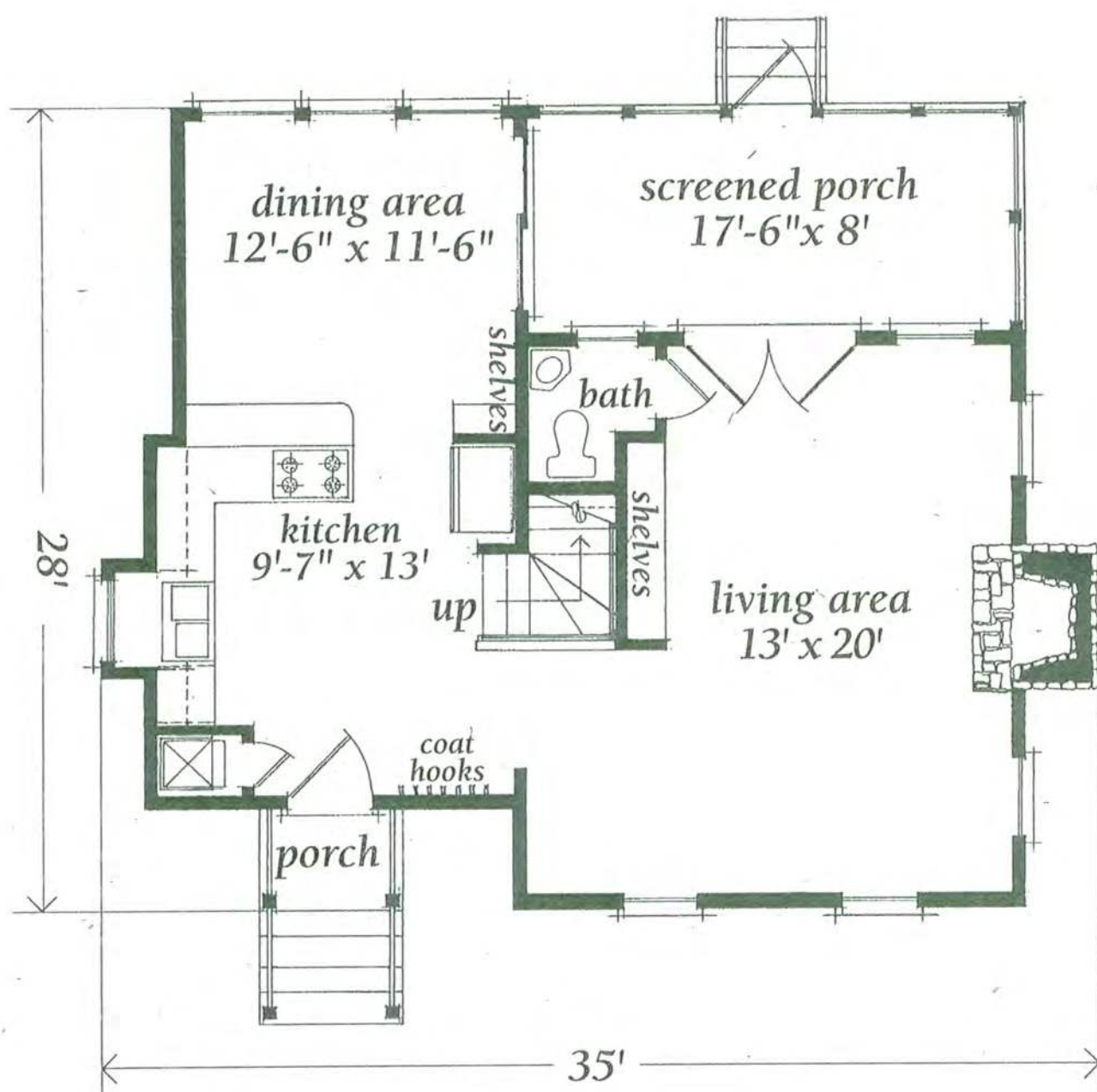
FIRST FLOOR (680 SQ. FT.)
