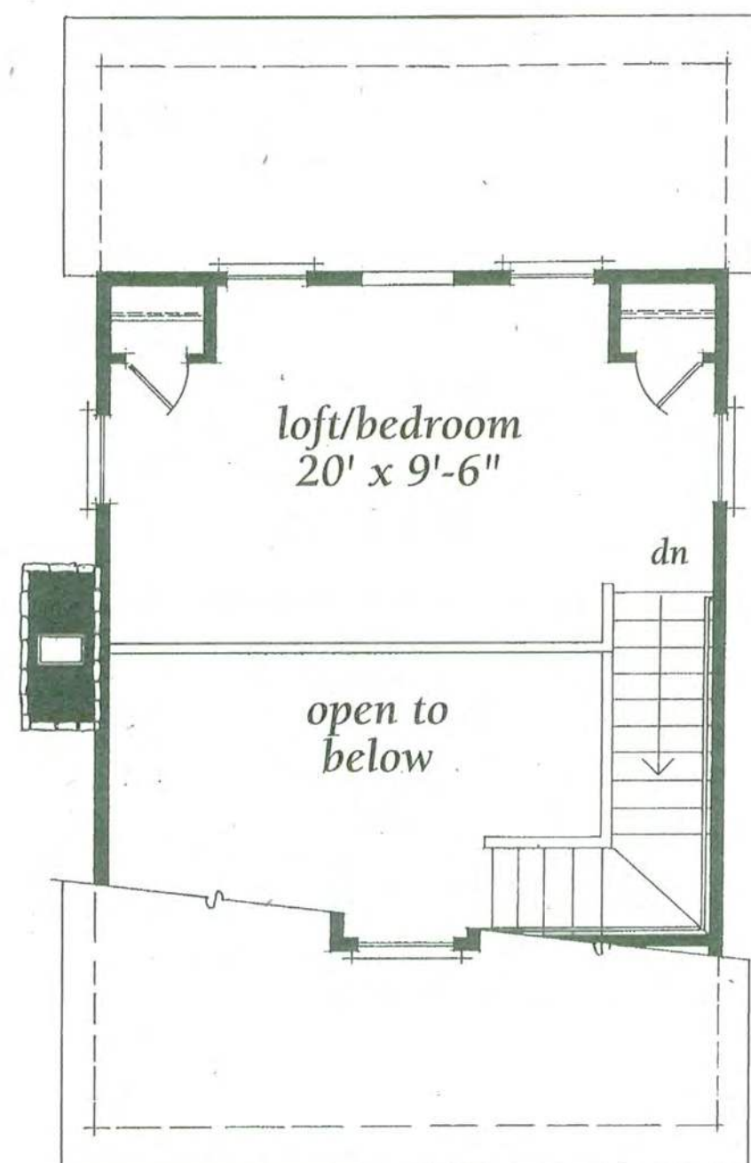
SECOND FLOOR (238 SQ. FT.)
