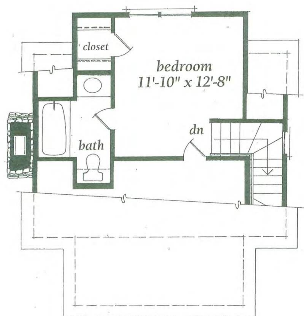
SECOND FLOOR (222 SQ. FT.)
