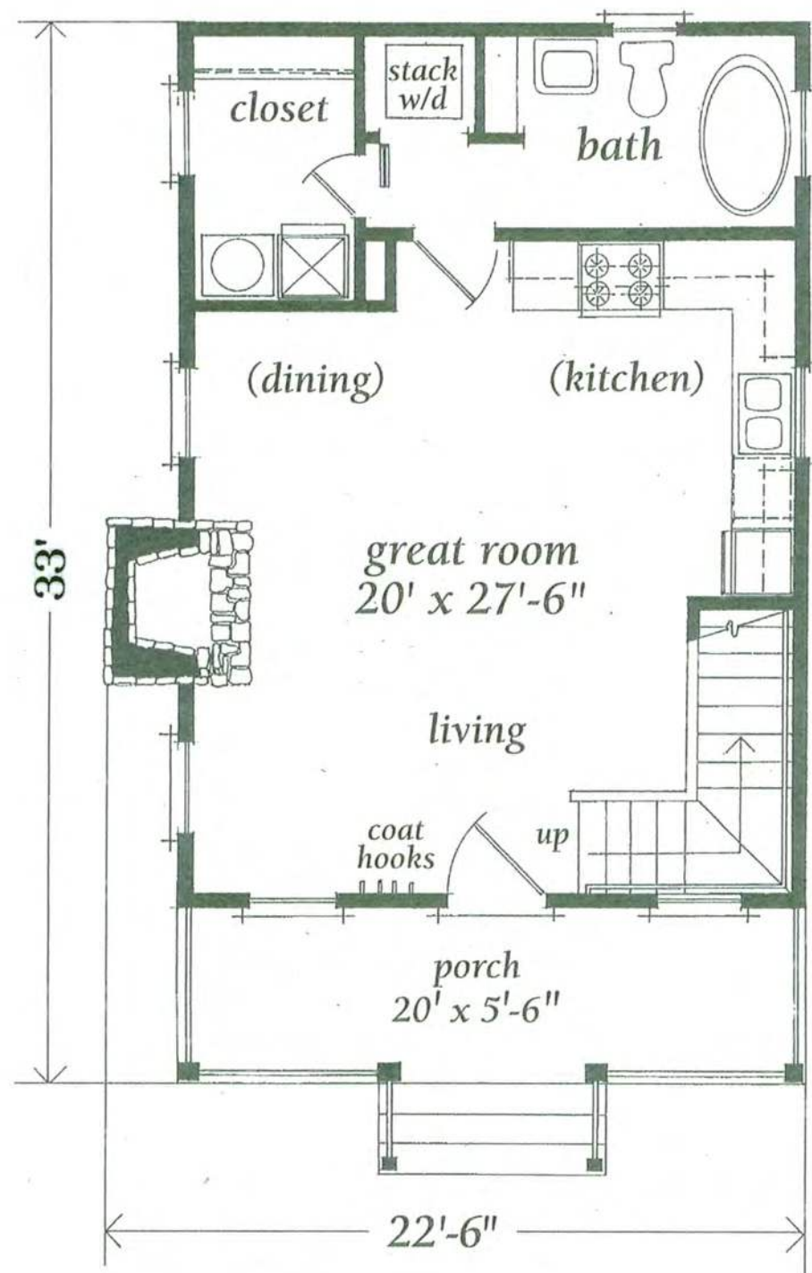
FIRST FLOOR (562 SQ. FT.)
